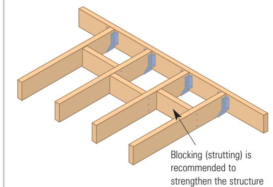
Figure 6a: Blocking joists
